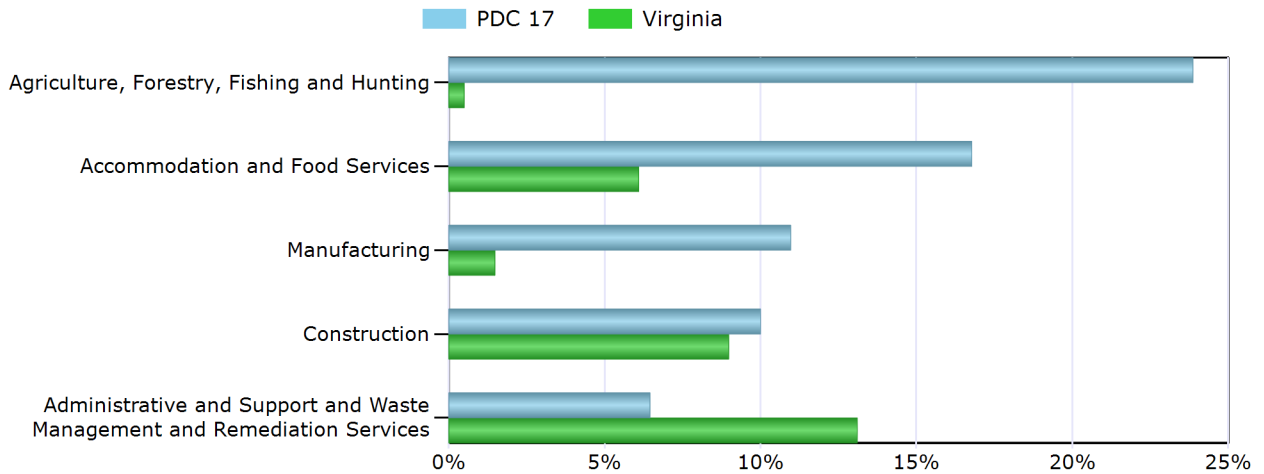
Top 5 Industries With Largest Number of Claimants in PDC 17 (excludes unclassified)
